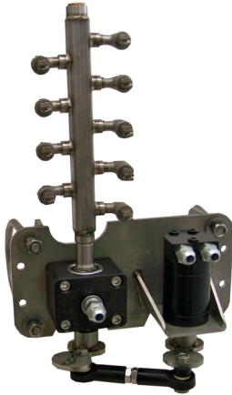
OSCILLATOR ASSEMBLY With SS Meg Nozzles $2,495.00
